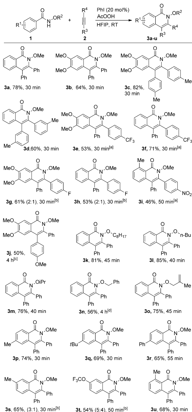
Scheme 2. Scope of the organocatalyzed annulation. Reaction conditions: 1 (0.15 mmol), 2 (0.18 mmol), 20 mol% PhI and AcOOH (1.5 equiv) in HFIP at room temperature. [a] 25 mol% of PhI was used. [b] Major isomer is shown. [c] PhI(OAc) 2 (1.5 equiv) used instead of PhI and AcOOH. [d] Catalyst A (10 mol%), CF 3 CO 2 H (5 equiv) and AcOOH (2 equiv) were used in 1,2-dichloroethane (2 mL).
